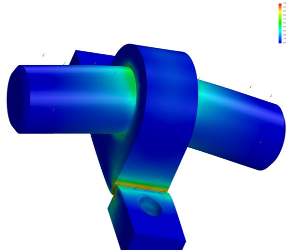
Pillow Block Assembly FEA SolidWorks
